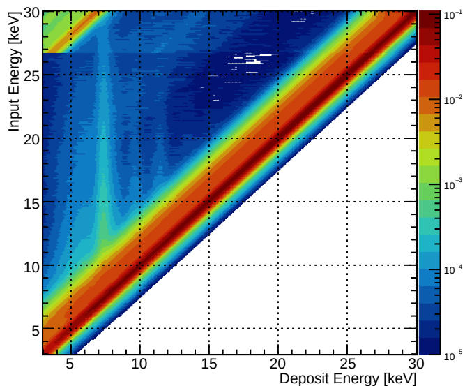
Response Matrix w Reso. + LET (1Hit)
