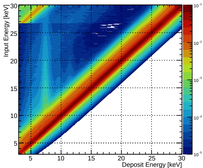
Response Matrix w Reso. + LET (Mix)
