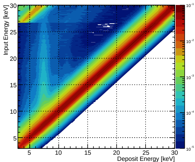
Response Matrix w Reso. + LET (2Hit)
