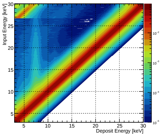
Response Matrix w Reso. (2Hit)
